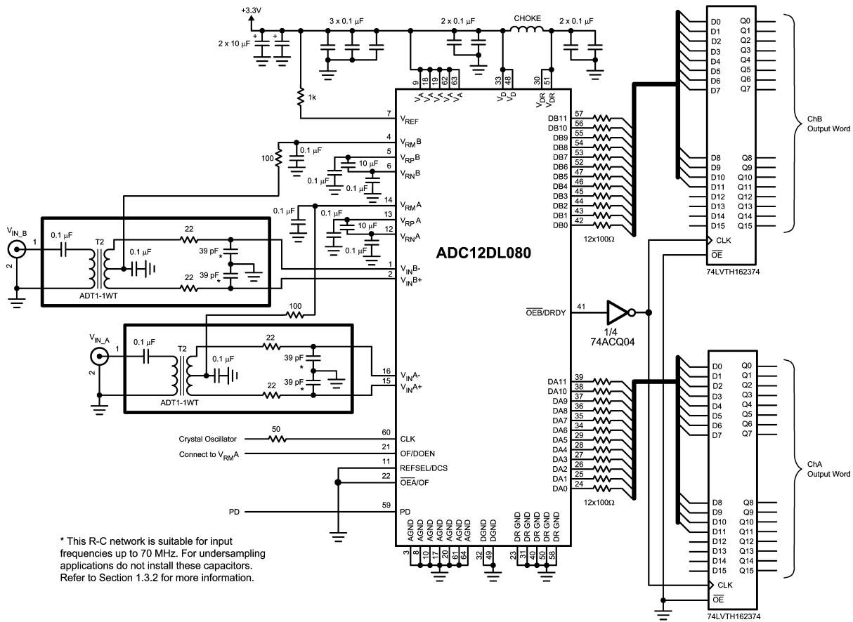
FIGURE 4. Application Circuit using Transformer Drive Circuit
